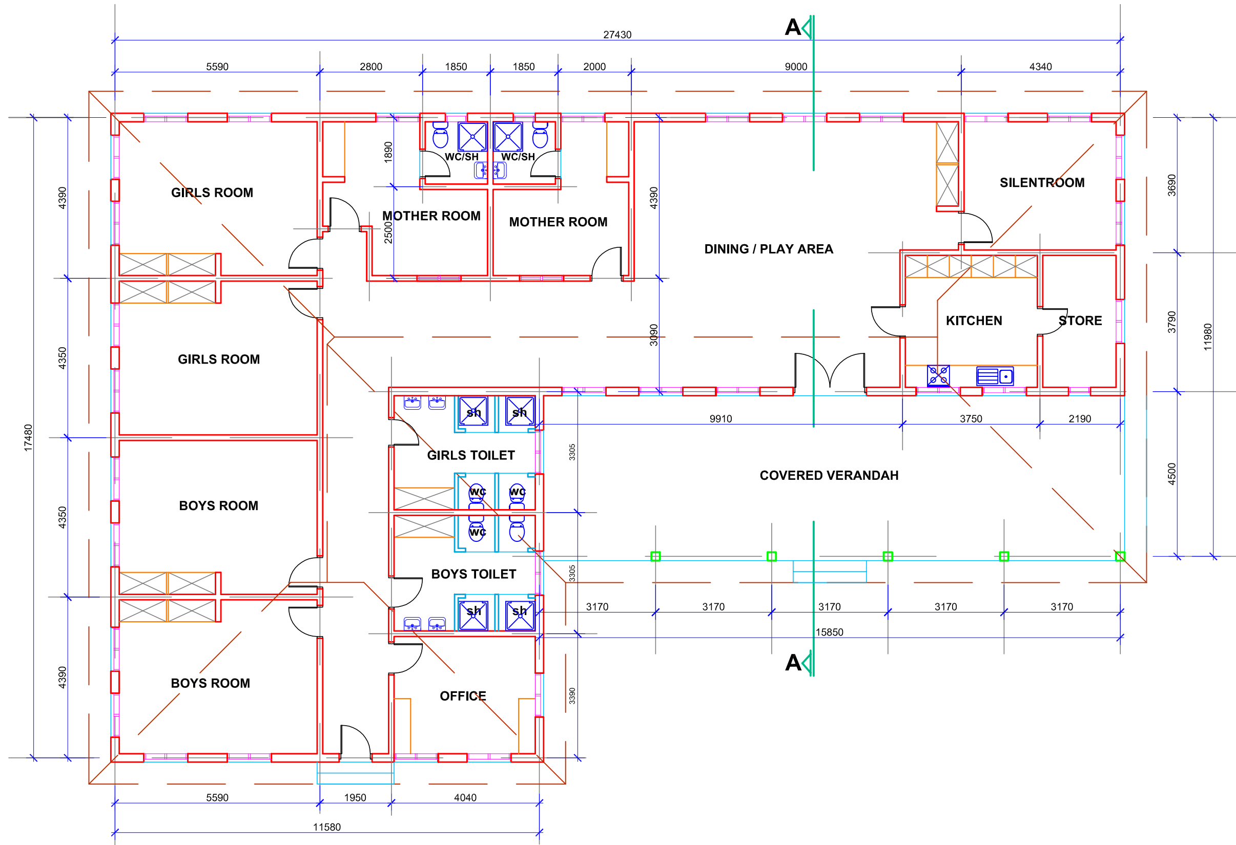
FLOOR PLAN
