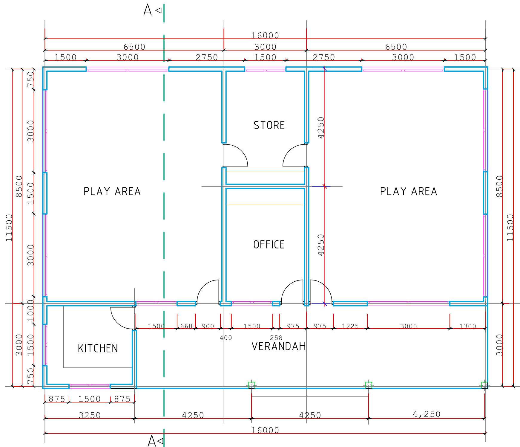
FLOOR PLAN-NURSERY BLOCK
